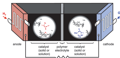
Figure 1. Direct observation of catalysts in a fuel cell [5] —an abstract depiction of a fuel cell. Water-saturated \text{H}_2 and \text{O}_2 gases flow through conduits in the electrodes (red and blue). In solution-phase experiments, water-soluble catalysts with the \text{NO}_3^- counteranion are dissolved in the gas conduits. In solid-phase experiments, water-insoluble catalysts with the \text{CF}_3\text{SO}_3^- counteranion are immobilized on carbon cloth sandwiched between the electrodes and the proton-conducting polymer electrolyte. Protons pass through the polymer electrolyte and electrons flow through an electrical circuit to the cathode.
